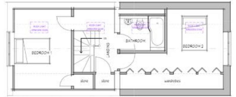
2 PROPOSED FIRST FLOOR LAYOUT PLAN
